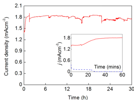
Figure 2. Bulk electrolysis of a 0.2 M solution of \text{Co}_3(\text{PO}_4)_2 in 1 M \text{H}_3\text{PO}_4 (final \text{pH} = 1.6 ) in a single chamber cell and a two-electrode configuration at room temperature. Both electrodes were ITO glass ( 7.5 \text{ cm}^2 ) and the effective cell voltage corrected for resistive losses was 2.2 V ( R = 61 \Omega ). Red line (main figure and inset): electrolysis in 0.2 M \text{Co}_3(\text{PO}_4)_2 . Blue dashed line (inset only): electrolysis under the same conditions but in the absence of Co(II). All current densities are based on the geometrical surface area of the electrodes.
