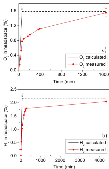
Figure 3. GCHA of airtight cells during and after electrolysis of a solution of 0.2 M Co 3 (PO 4 ) 2 in 1 M H 3 PO 4 at pH 1.6. Black solid lines indicate the % of a given gas expected in the cell headspace based on the charge passed during electrolysis (20 C was passed in both cases). Red circles indicate actual measurements of the percent of each gas in the cell headspace as deposited films slowly dissolved. Solid red lines and black dashed lines are provided as guides to the eye. Arrows indicate where electrolysis was stopped. (a) Oxygen evolution into the cell headspace. (b) Hydrogen evolution data.
