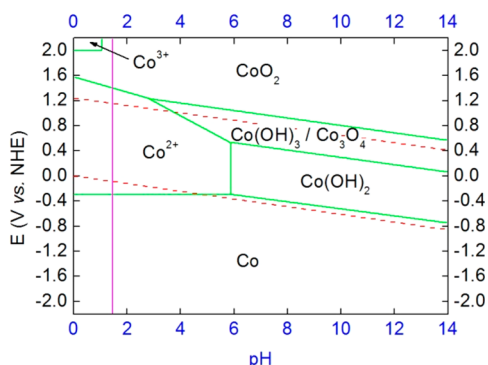
Figure 1. Simplified Pourbaix diagram for cobalt in aqueous solution. Green lines represent the borders of thermodynamic stability of the various species (adapted from ref 24). Dissolved species are considered as having an activity of 1. Red dashed lines mark the region of water stability, the lower line corresponding to the hydrogen evolution reaction and the upper line to the oxygen evolution reaction. The vertical magenta line is drawn at \text{pH} = 1.6 as a guide to the eye.
