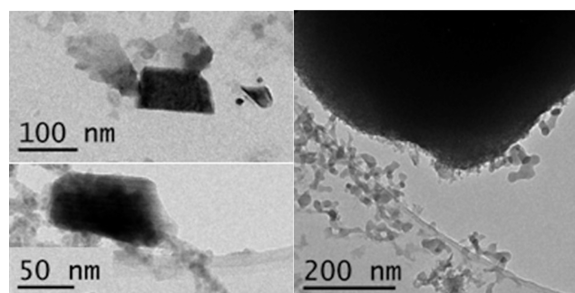
Figure 5. TEM images of particles from the anode compartment of electrolysis cells containing 0.2 M \text{Co}_3(\text{PO}_4)_2 at pH 1.6. A two-electrode configuration was used, and both electrodes were ITO. The effective cell voltage was 2.4 V.
