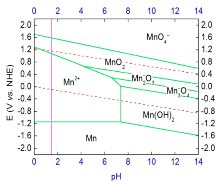
Figure 6. Simplified Pourbaix diagram for manganese in aqueous solution. Green lines represent the borders of thermodynamic stability of the various species (adapted from ref 24). Dissolved species are considered as having an activity of 1. Red dashed lines mark the region of water stability, the lower line corresponding to the hydrogen evolution reaction and the upper line to the oxygen evolution reaction. The vertical magenta line is drawn at \text{pH} = 1.6 as a guide to the eye.
