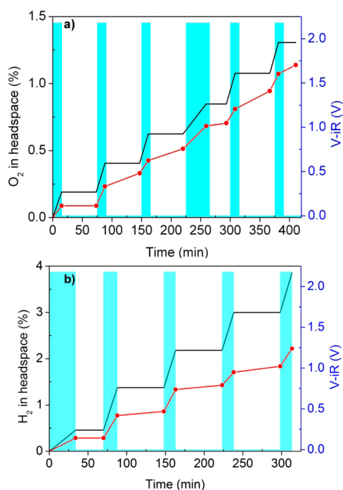
Figure 4. GCHA of airtight cells where electrolysis of a solution of 0.2 M \text{Co}_3(\text{PO}_4)_2 in 1 M \text{H}_3\text{PO}_4 at pH 1.6 has been stopped and restarted several times and the headspace of the cell sampled. Black solid lines (left-hand y-axis) indicate the % of oxygen or hydrogen expected in the cell headspace based on the charge passed during electrolysis. Red circles and red lines indicate actual measurements of the percent of oxygen or hydrogen in the cell headspace. The blue shaded areas (whose associated y-axis is on the right-hand side) indicate when an effective voltage of 2.2 V was applied and thus when electrolysis was occurring. (a) Oxygen evolution into the cell headspace, R = 129 \Omega . (b) Hydrogen evolution data, R = 125 \Omega .
